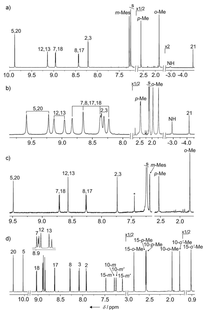
Figure 3. 1 H NMR spectra of a) 6 (300 K, [D]chloroform), b) 6 (190 K, [D 8 ]toluene), c) 6-Pd (300 K, [D]chloroform), and d) 11 (300 K, [D 2 ]dichloromethane). Atom assignments correspond to the systematic position numbering or denote proton groups such as o -, m -, p -positions of the meso-mesityl groups.
