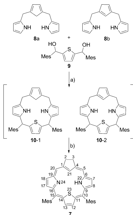
Scheme 3. Synthesis of 7 . Reaction conditions: a) \text{BF}_3 \cdot \text{Et}_2\text{O} (1 equiv), 3% EtOH in \text{CHCl}_3 , RT, 1 h; b) triethylamine (1.2 equiv), p -chloranil (6 equiv), RT, 1 h. Mes = mesityl = 2,4,6-trimethylphenyl.
