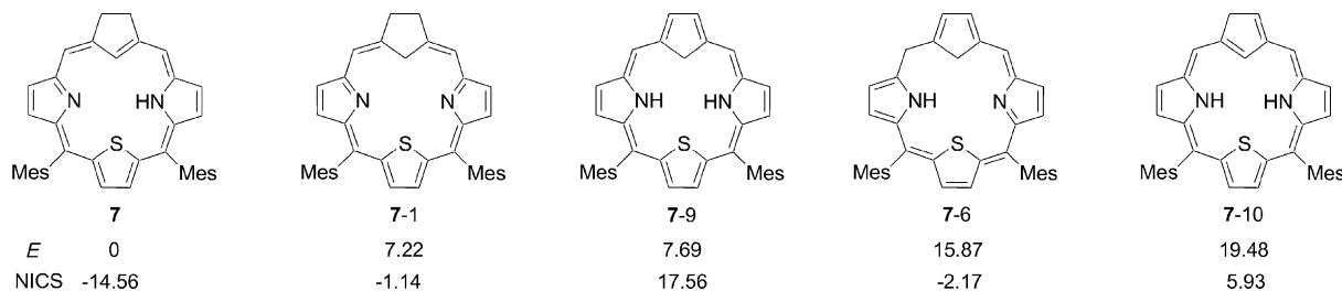
Figure 6. Geometries, calculated energies (in kcal mol ^{-1} ), and NICS values (in ppm) of chosen dihydro-10,15-dimesityl-21-carba-23-thiaporphyrin isomers obtained by DFT optimization.
