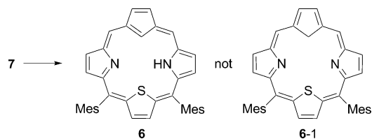
Scheme 4. Oxidation of 7 : [\text{D}]\text{chloroform} , DDQ (1 equiv) dissolved in [\text{D}_6]\text{benzene} , RT, 20 min.
