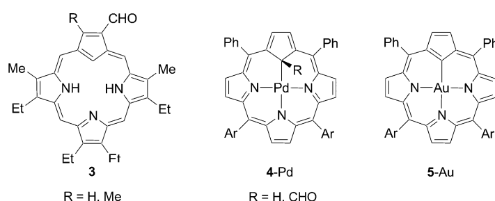
Scheme 2. True carbaporphyrins reported to date.
