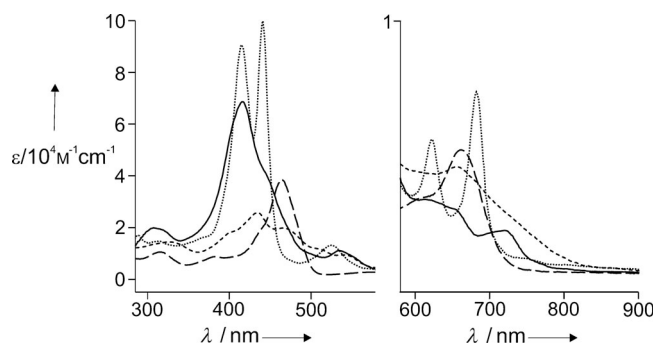
Figure 2. The electronic spectra of 6 (solid line), 7 (dotted line), 6-Pd (short dashed line), and 7-Pd (long dashed line) in dichloromethane.
