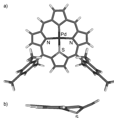
Figure 5. DFT-optimized structure of 6-Pd : a) perspective view and b) side view (mesityl groups at the 10- and 15-positions are omitted for clarity). Selected bond lengths [Å]: Pd-C(21) 1.96, Pd-N(22) 2.09, Pd-N(24) 2.09, Pd-S(23) 2.32. The angle between the plane of the thiophene ring and the plane of four \text{C}_{\text{meso}} atoms is 30.0°.
