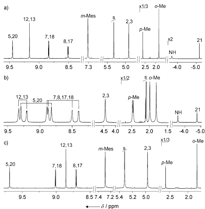
Figure 4. ^1\text{H} NMR spectra of a) 7 (300 K, [\text{D}_2] dichloromethane), b) 7 (190 K, [\text{D}_8] toluene) and c) 7-Pd (300 K, [\text{D}_2] dichloromethane). Atom assignments correspond to the systematic position numbering or denote proton groups such as o -, m -, p -positions of the meso-mesityl groups.
