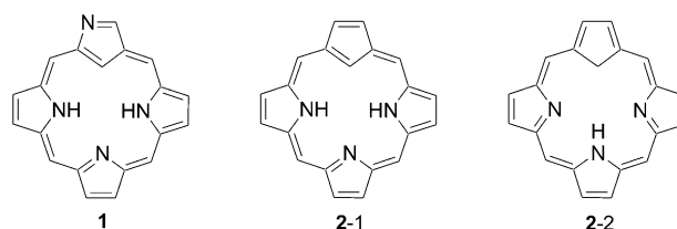
Scheme 1. N-Confused porphyrin 1 and true carbaporphyrins 2 .
