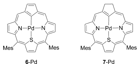
Scheme 5. Palladium(II) complexes of carbathiaporphyrin ( 6-Pd ) and carbathiachlorin ( 7-Pd ).
