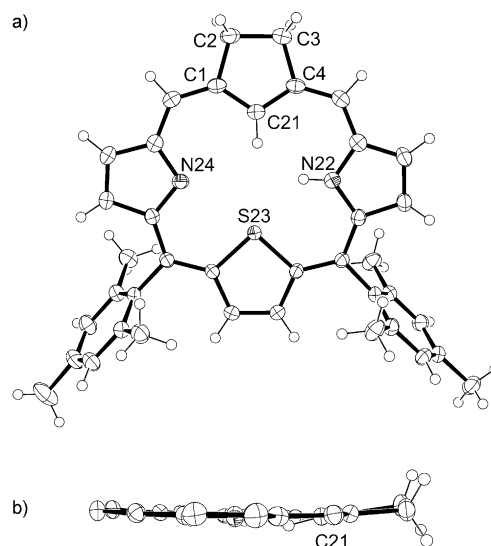
Figure 1. Molecular structure of carbathiachlorin 7 : a) perspective view and b) side view (mesityl groups and selected H atoms are omitted for clarity). The vibrational ellipsoids represent 50% probability. Selected bond lengths [Å]: C1–C2 1.515(3), C2–C3 1.536(3), C3–C4 1.524(3), C1–C21 1.403(3), C4–C21 1.404(3).
